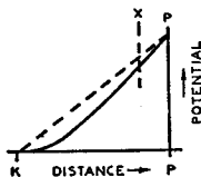
Fig. 7—Effect of space charge on potential distribution in a diode.
